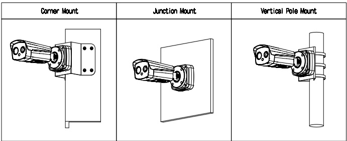
PFA151A + PFA121A Corner Mount Bracket
