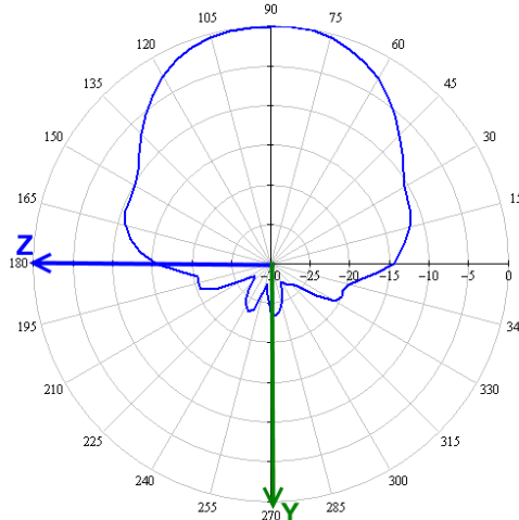
ELEVATION (YZ)
