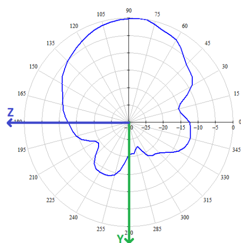
ELEVATION (YZ)
