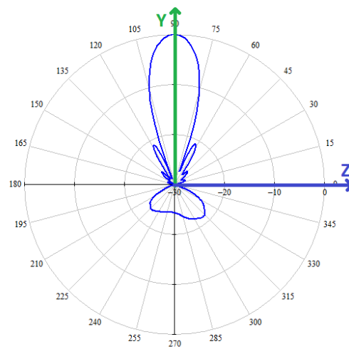
ELEVATION (YZ)
