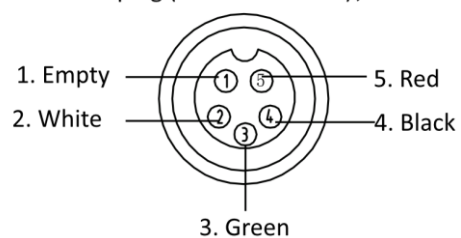
5-Pin Aviation Plug Front Panel
