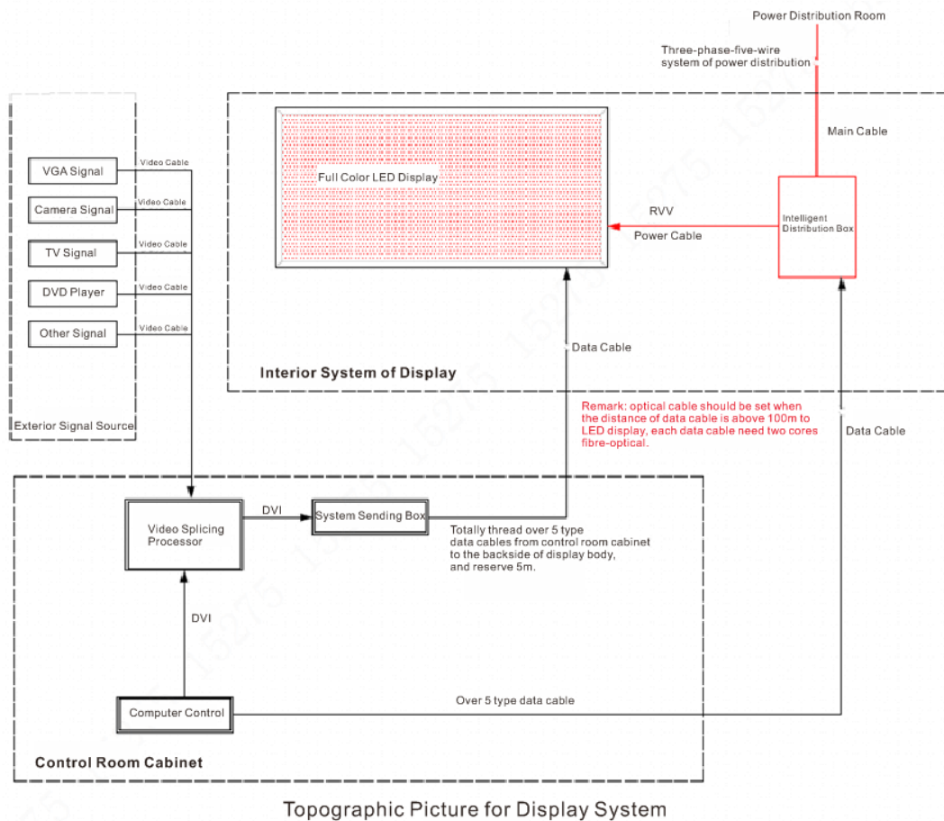
Picture 4-2-1 Diagram for Connection
