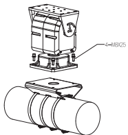
3702 Pole Mount Bracket (purchase separately)
