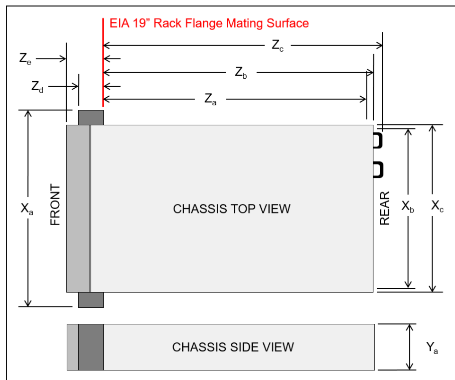
Figure 23. Server dimensions
