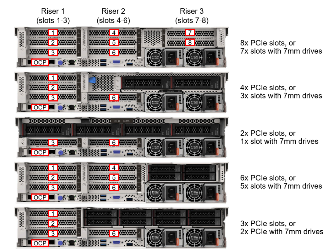
Figure 14. SR650 V2 slot configurations
