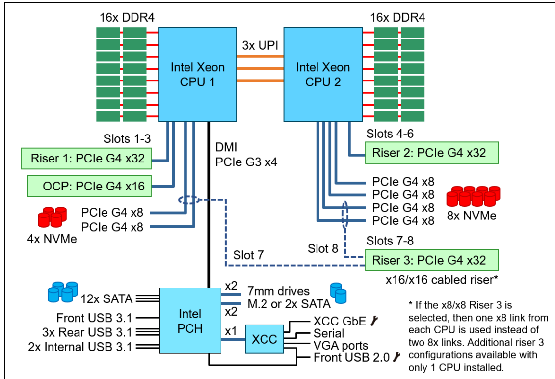
Figure 5. SR650 V2 system architectural block diagram
